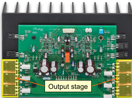
E-650 Power Amplifier Module
